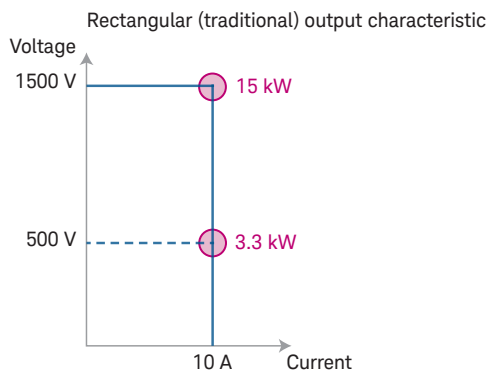
Figure 5. Rectangular output characteristic
