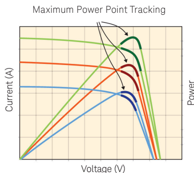
Maximum Power Point Tracking with varying levels of irradiance
